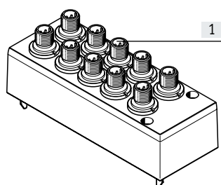
[1] 1xM12 plug, 5-pin
