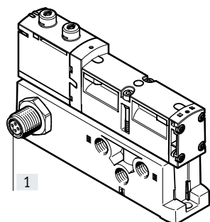
[1] 1xM12 plug, 4-pin to EN 61076-2-101
