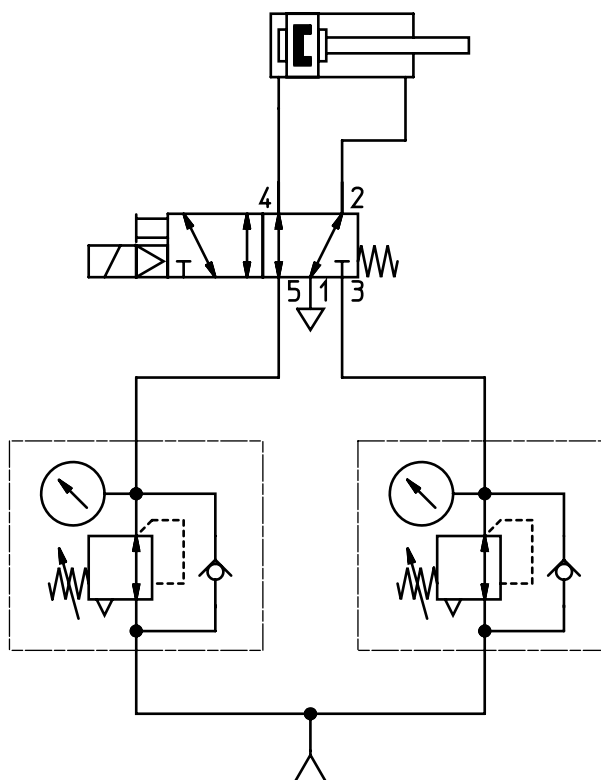
Dual-pressure operation with reversible controller
