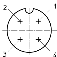
[1] 1xM12 plug, 4-pin to EN 61076-2-101
